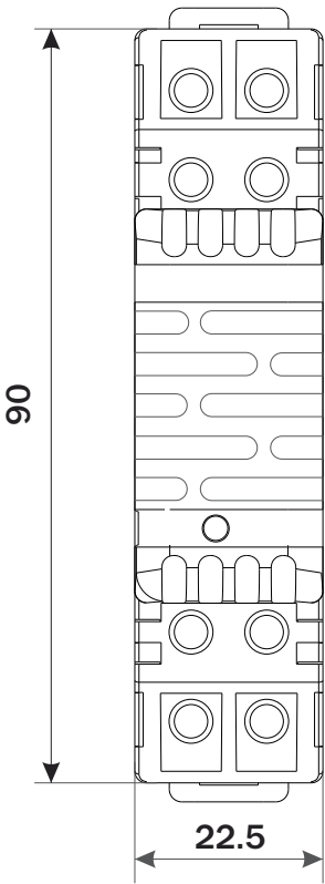
FRONT VIEW
