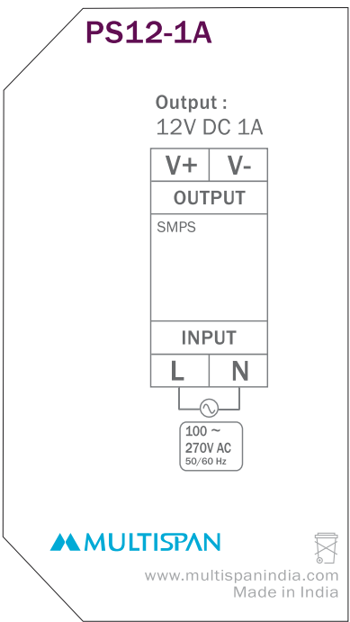
PS12-1A Switch Mode Power Supply
